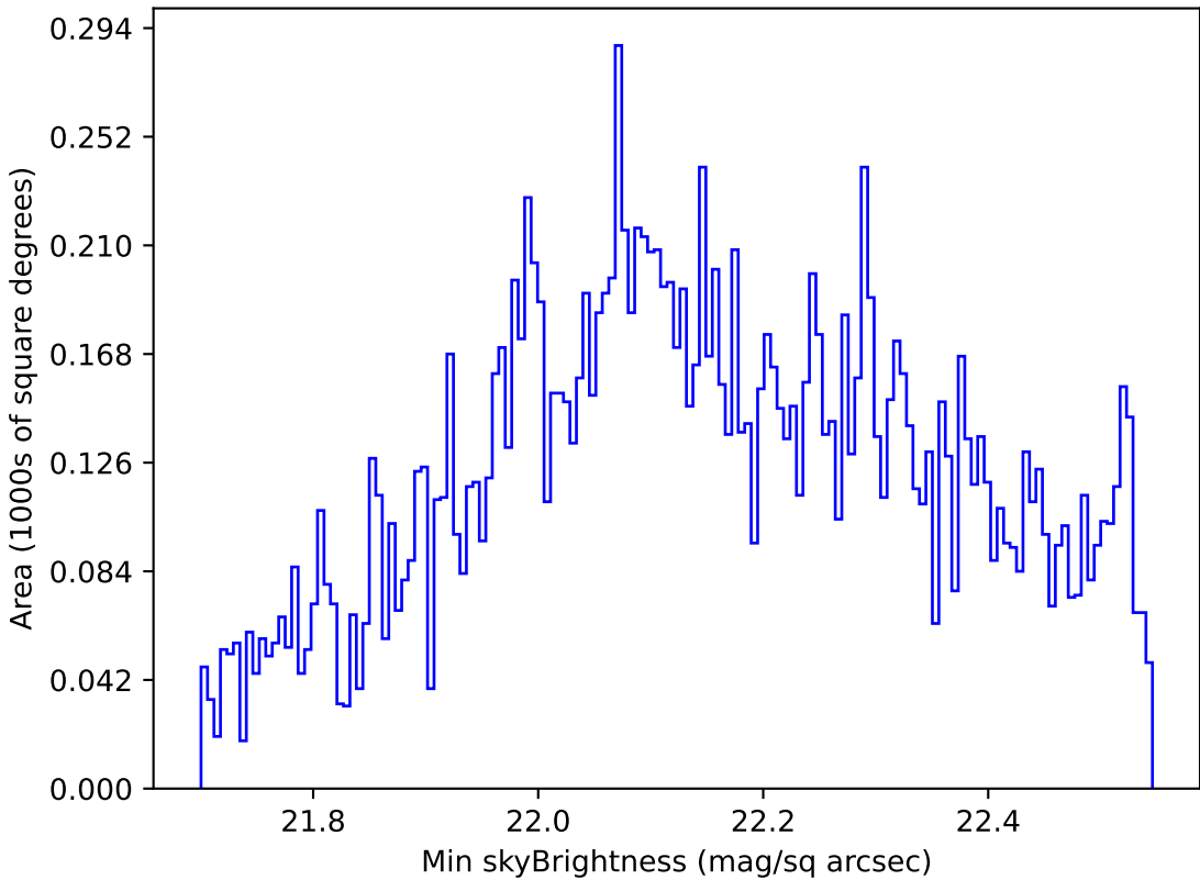
too_elab_heavy_r64_d2_ugrizy_v3.4_10yrs WFD u band: Min skyBrightness
