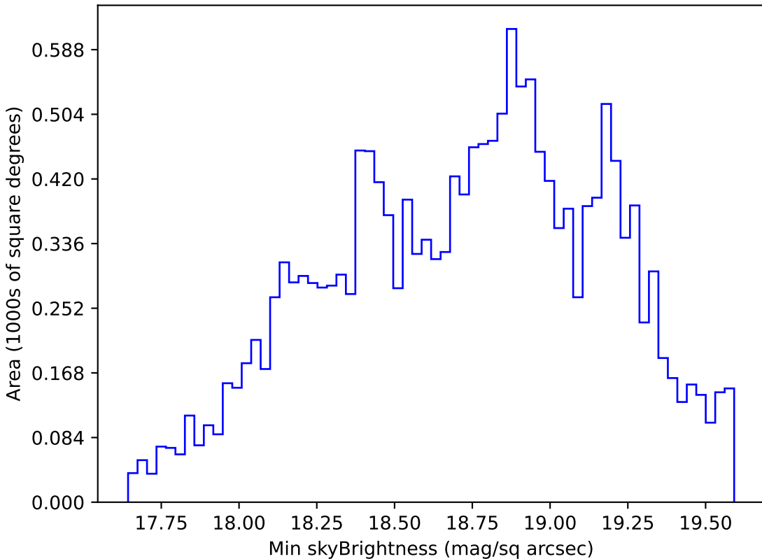
too_elab_heavy_r64_d2_ugrizy_v3.4_10yrs WFD r band: Min skyBrightness
