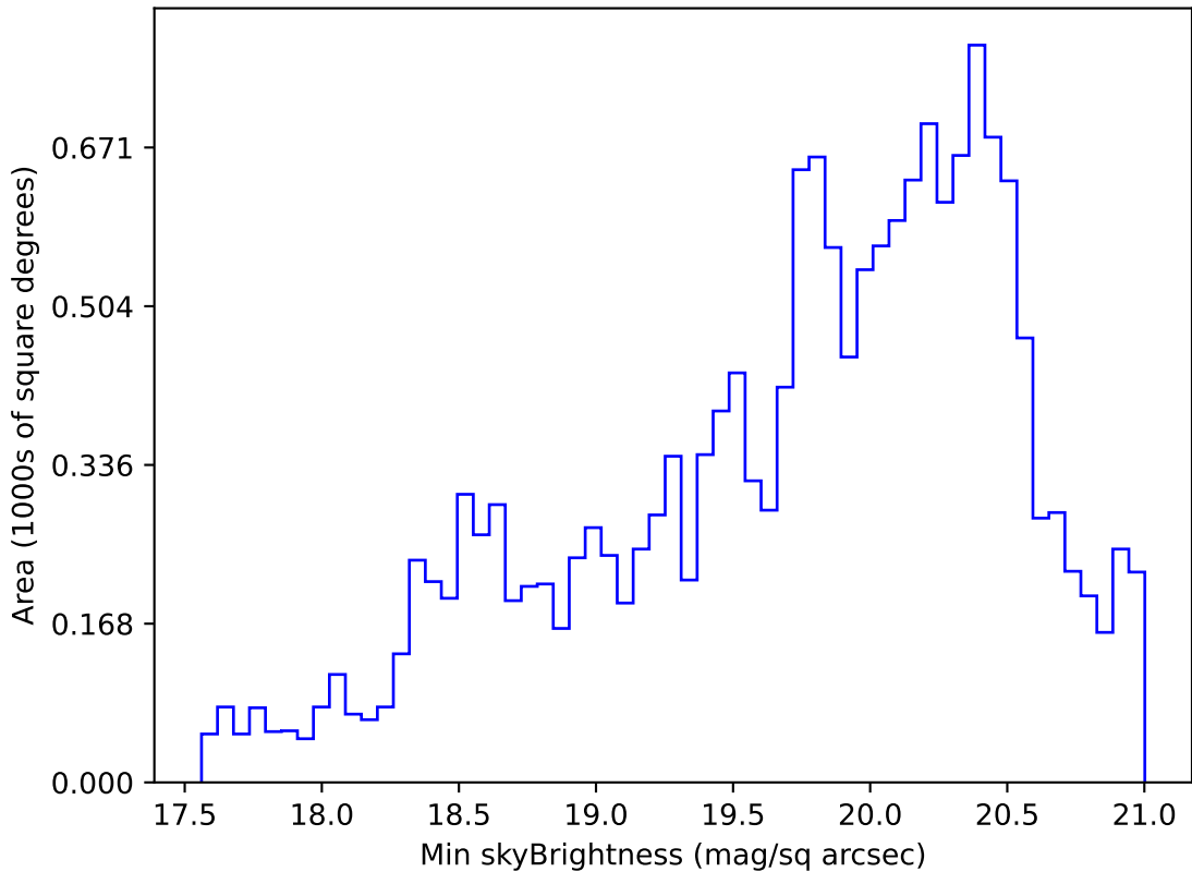
too_elab_heavy_r64_d2_ugrizy_v3.4_10yrs WFD g band: Min skyBrightness
