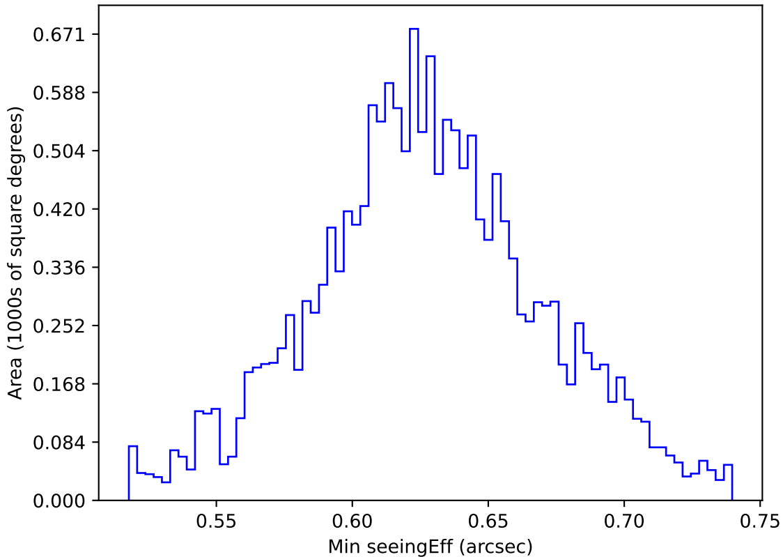
too_elab_heavy_r64_d2_ugrizy_v3.4_10yrs WFD y band: Min seeingEff
