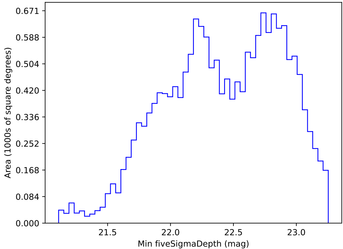
too_elab_heavy_r64_d2_ugrizy_v3.4_10yrs WFD r band: Min fiveSigmaDepth
