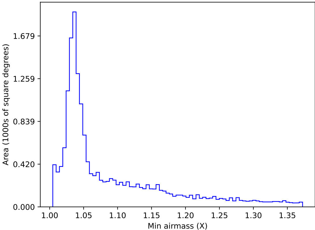
too_elab_heavy_r64_d2_ugrizy_v3.4_10yrs WFD g band: Min airmass
