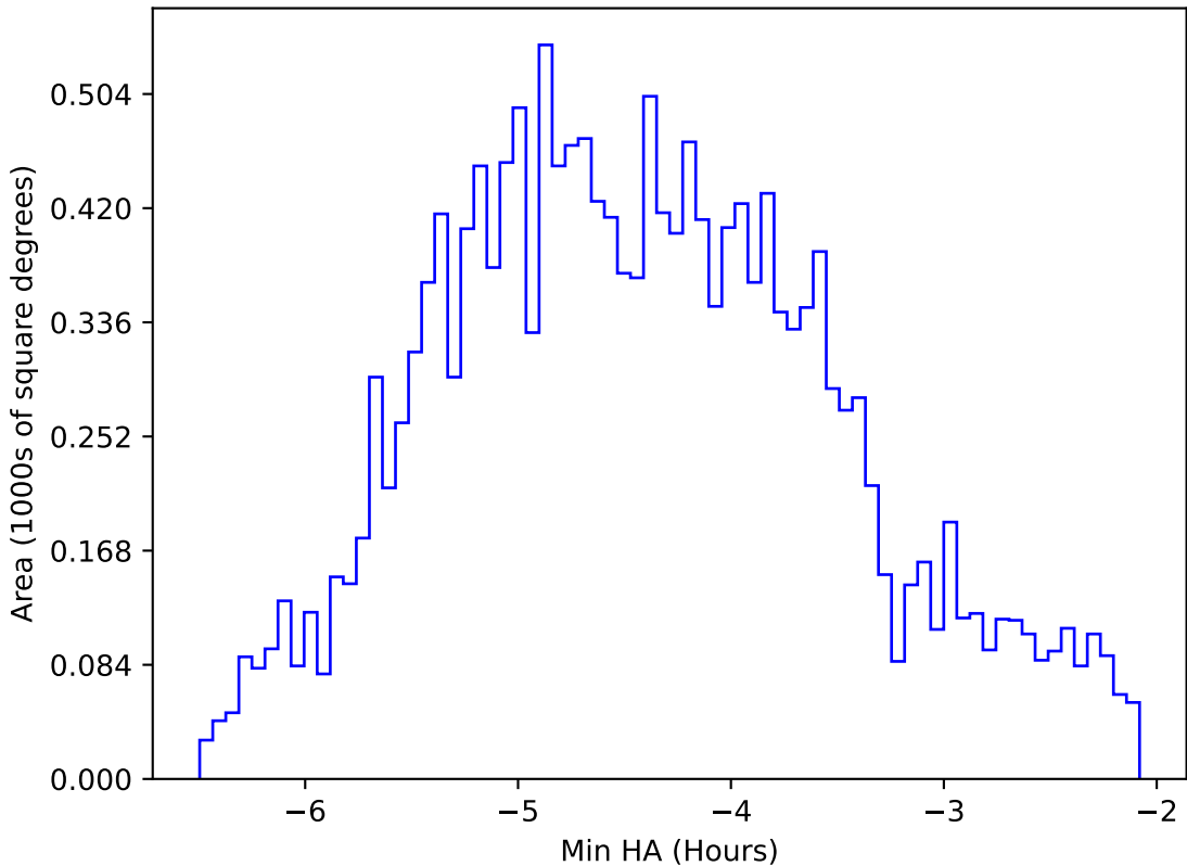
too_elab_heavy_r64_d2_ugrizy_v3.4_10yrs WFD z band: Min HA
