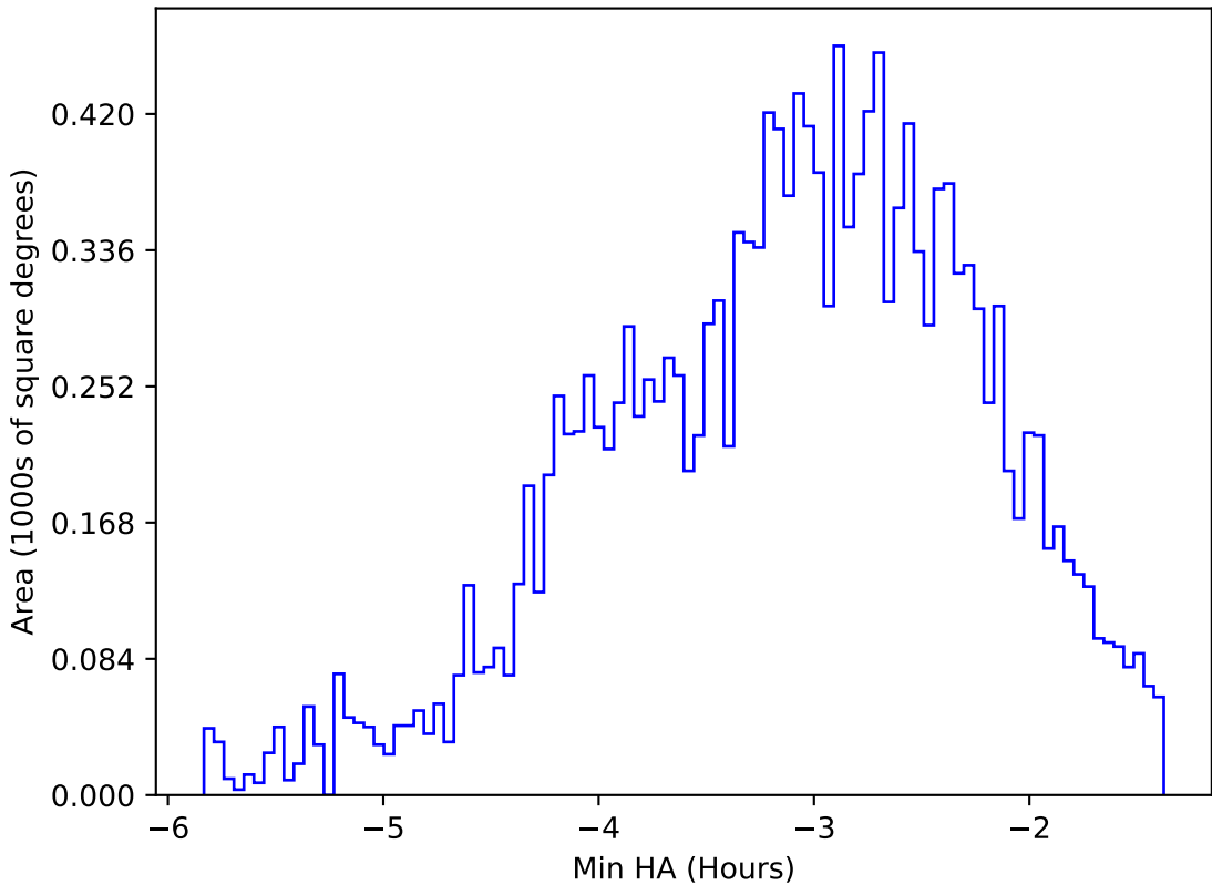
too_elab_heavy_r64_d2_ugrizy_v3.4_10yrs WFD u band: Min HA
