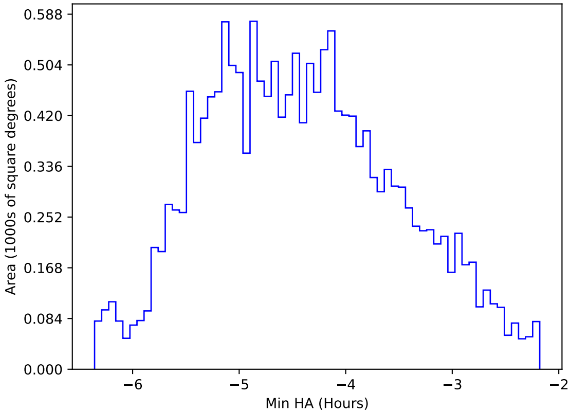
too_elab_heavy_r64_d2_ugrizy_v3.4_10yrs WFD r band: Min HA
