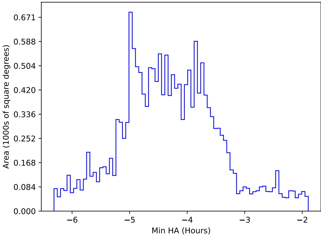
too_elab_heavy_r64_d2_ugrizy_v3.4_10yrs WFD g band: Min HA
