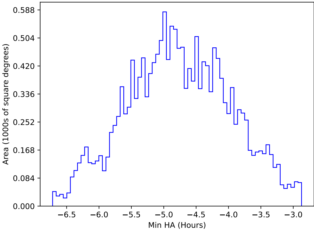
too_elab_heavy_r64_d2_ugrizy_v3.4_10yrs WFD all bands: Min HA
