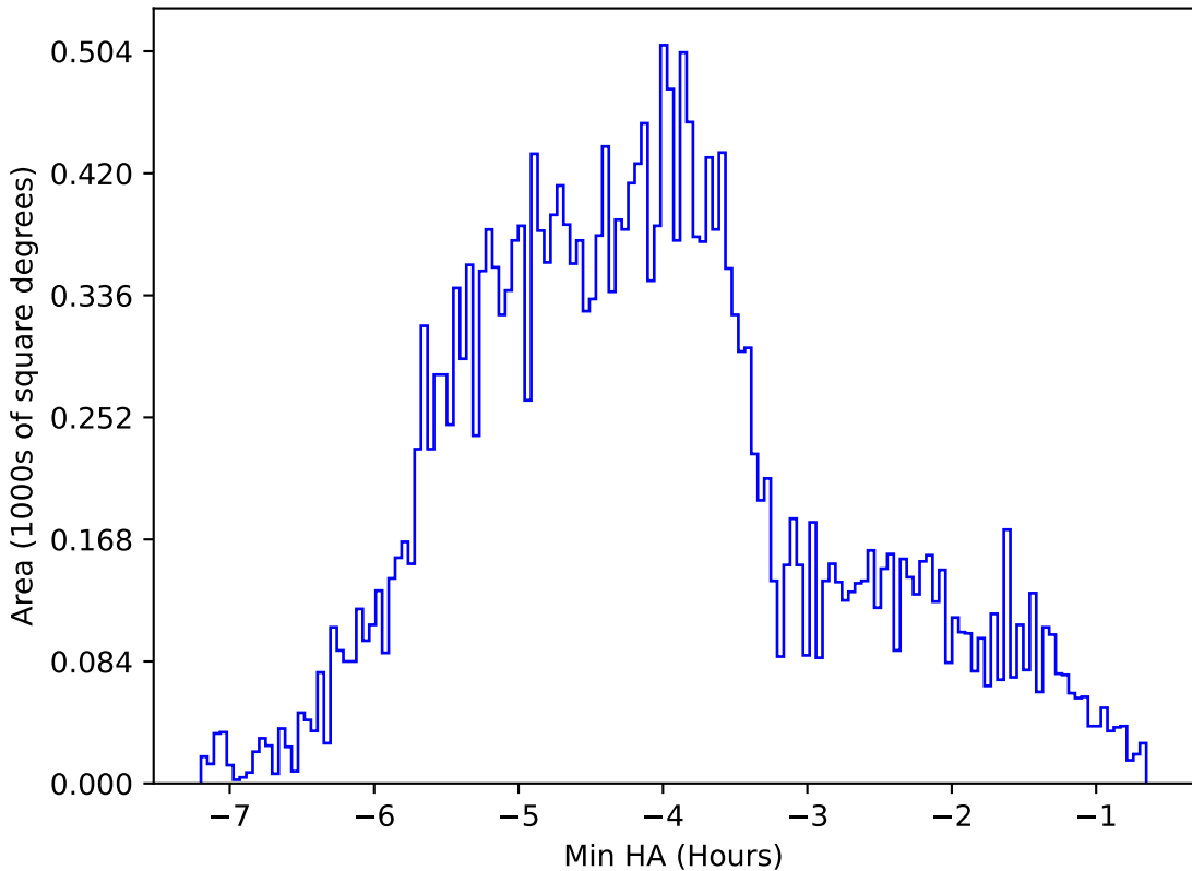
too_elab_heavy_r64_d2_ugrizy_v3.4_10yrs All sky z band: Min HA
