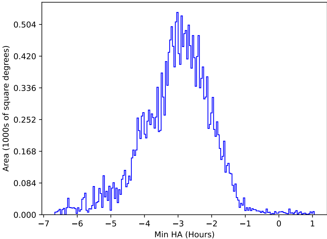
too_elab_heavy_r64_d2_ugrizy_v3.4_10yrs All sky u band: Min HA
