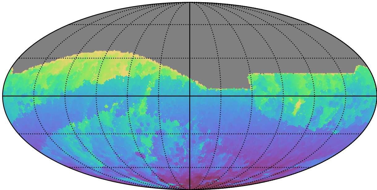
too_elab_heavy_r64_d2_ugrizy_v3.4_10yrs All sky r band: Min HA
