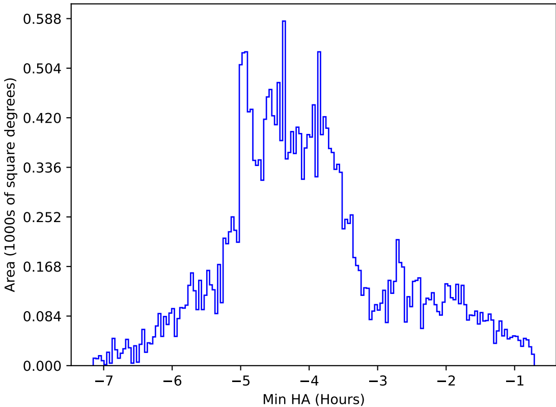
too_elab_heavy_r64_d2_ugrizy_v3.4_10yrs All sky g band: Min HA
