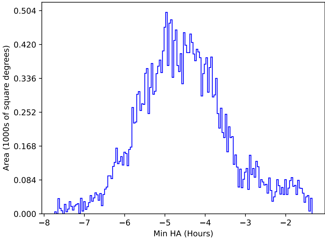
too_elab_heavy_r64_d2_ugrizy_v3.4_10yrs All sky all bands: Min HA
