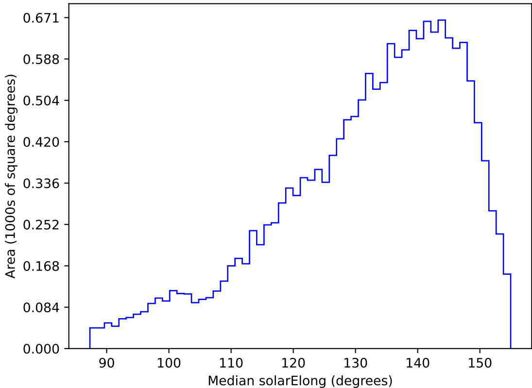
too_elab_heavy_r64_d2_ugrizy_v3.4_10yrs WFD u band: Median solarElong
