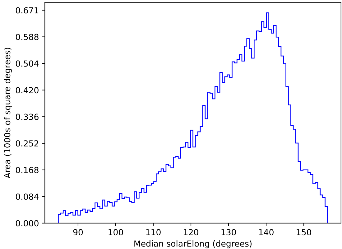
too_elab_heavy_r64_d2_ugrizy_v3.4_10yrs All sky r band: Median solarElong
