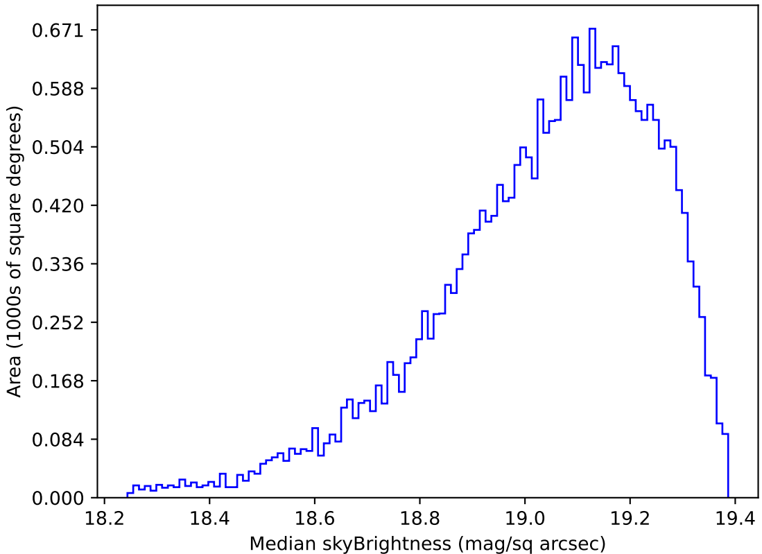
too_elab_heavy_r64_d2_ugrizy_v3.4_10yrs Yr 1 z band: Median skyBrightness
