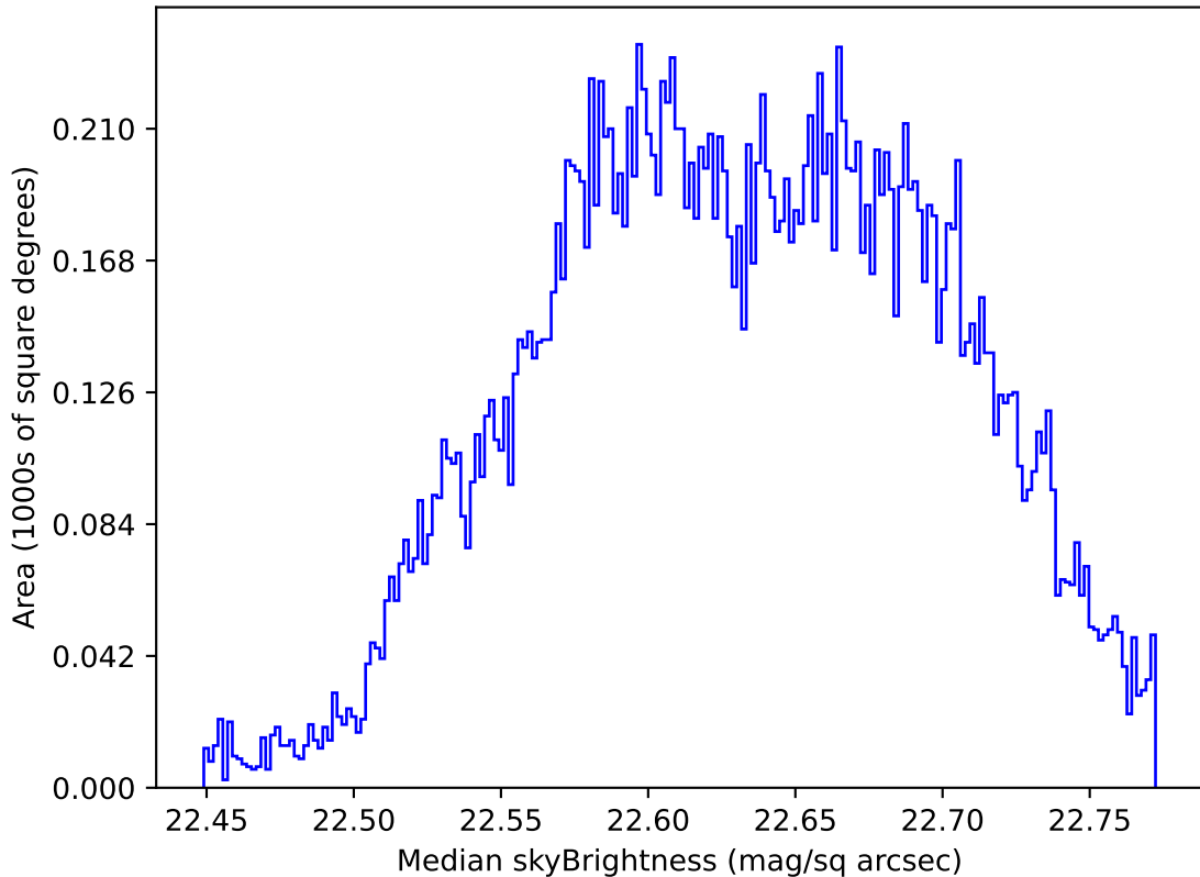
too_elab_heavy_r64_d2_ugrizy_v3.4_10yrs Yr 1 u band: Median skyBrightness
