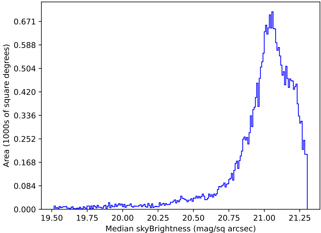
too_elab_heavy_r64_d2_ugrizy_v3.4_10yrs Yr 1 r band: Median skyBrightness
