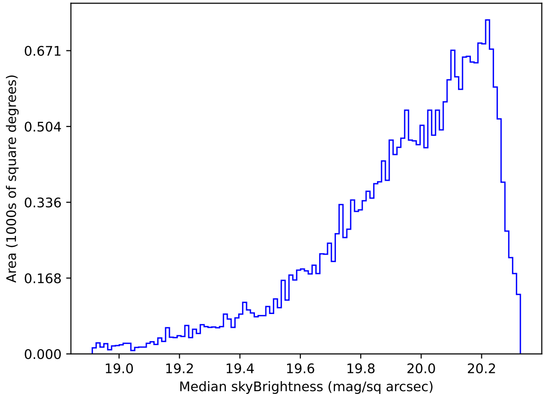
too_elab_heavy_r64_d2_ugrizy_v3.4_10yrs Yr 1 i band: Median skyBrightness
