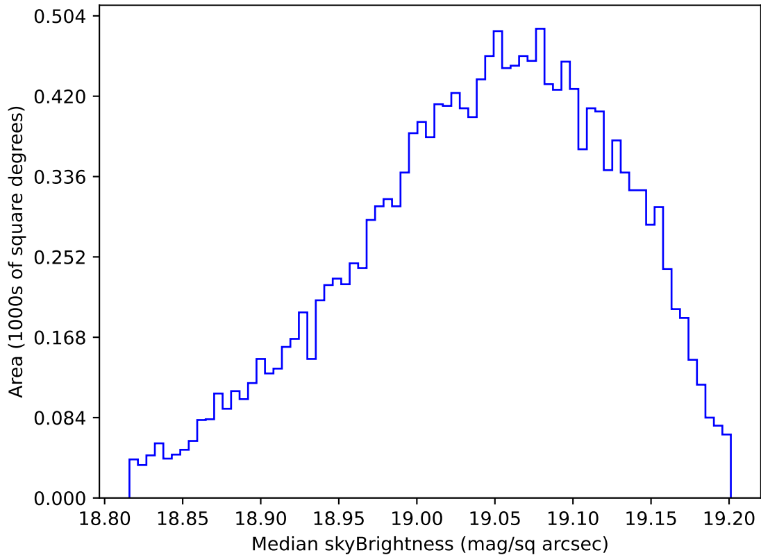
too_elab_heavy_r64_d2_ugrizy_v3.4_10yrs WFD z band: Median skyBrightness
