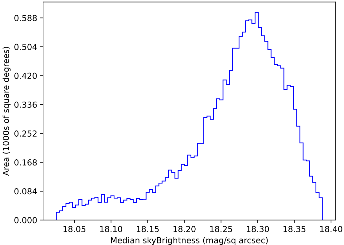
too_elab_heavy_r64_d2_ugrizy_v3.4_10yrs WFD y band: Median skyBrightness
