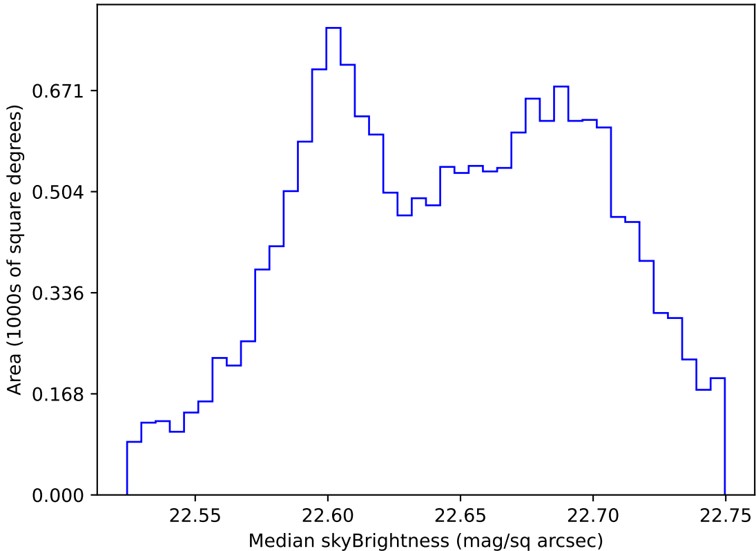
too_elab_heavy_r64_d2_ugrizy_v3.4_10yrs WFD u band: Median skyBrightness
