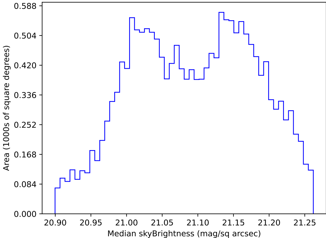
too_elab_heavy_r64_d2_ugrizy_v3.4_10yrs WFD r band: Median skyBrightness
