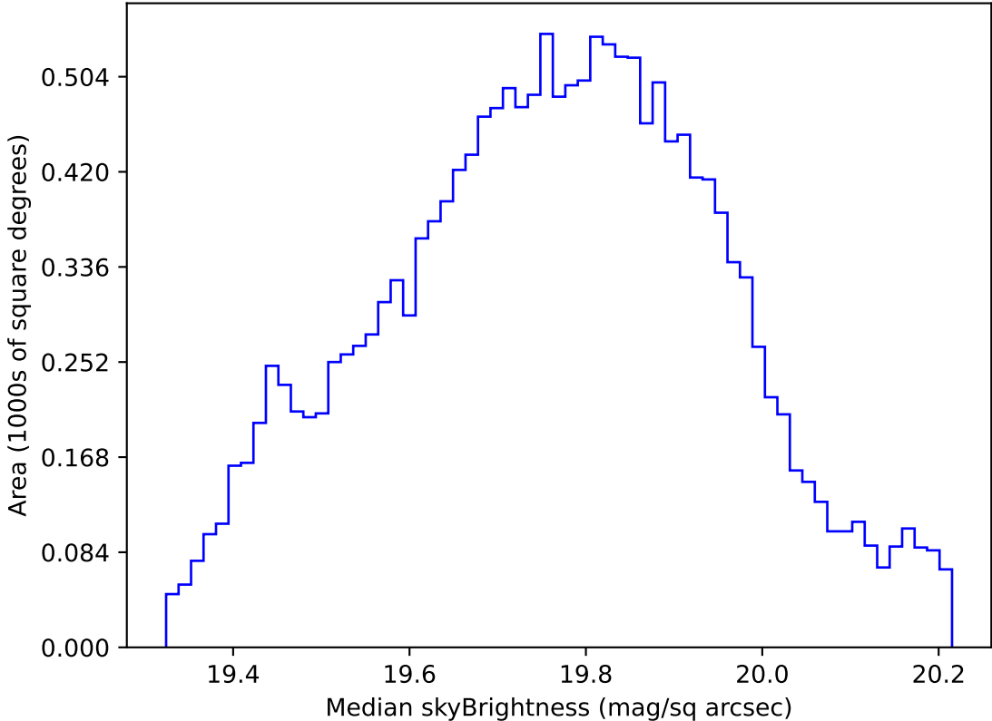
too_elab_heavy_r64_d2_ugrizy_v3.4_10yrs WFD all bands: Median skyBrightness
