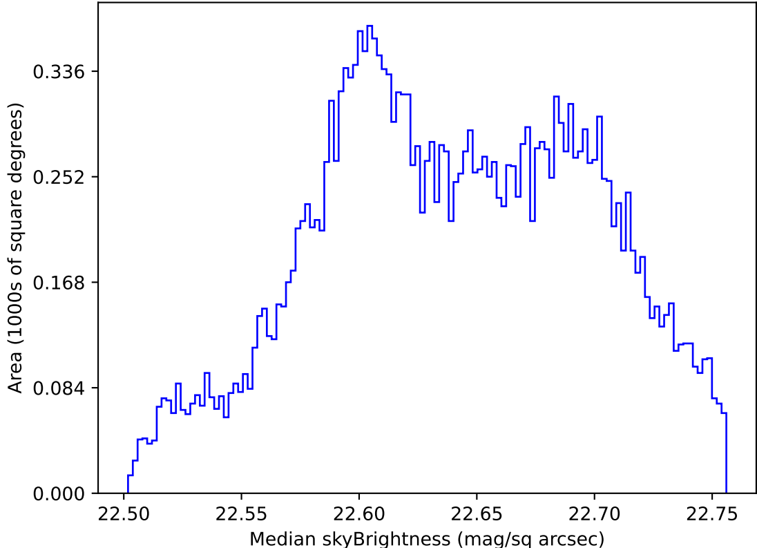
too_elab_heavy_r64_d2_ugrizy_v3.4_10yrs All sky u band: Median skyBrightness
