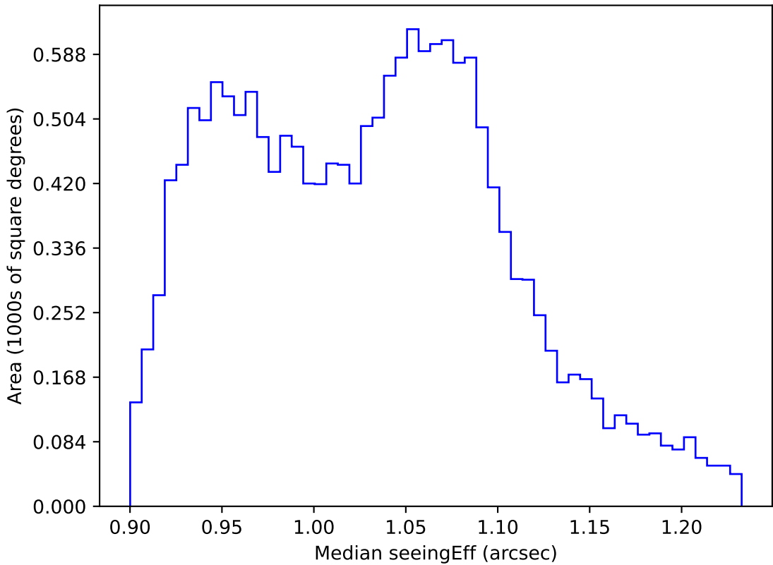
too_elab_heavy_r64_d2_ugrizy_v3.4_10yrs WFD all bands: Median seeingEff
