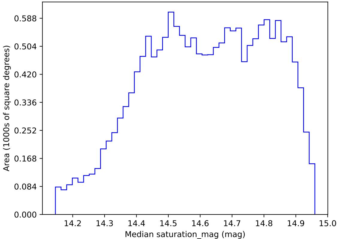
too_elab_heavy_r64_d2_ugrizy_v3.4_10yrs WFD r band: Median saturation_mag
