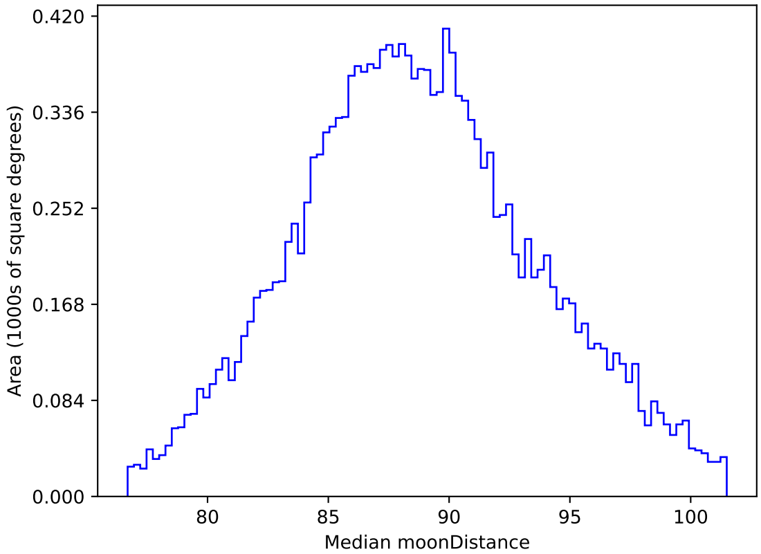
too_elab_heavy_r64_d2_ugrizy_v3.4_10yrs WFD all bands: Median moonDistance
