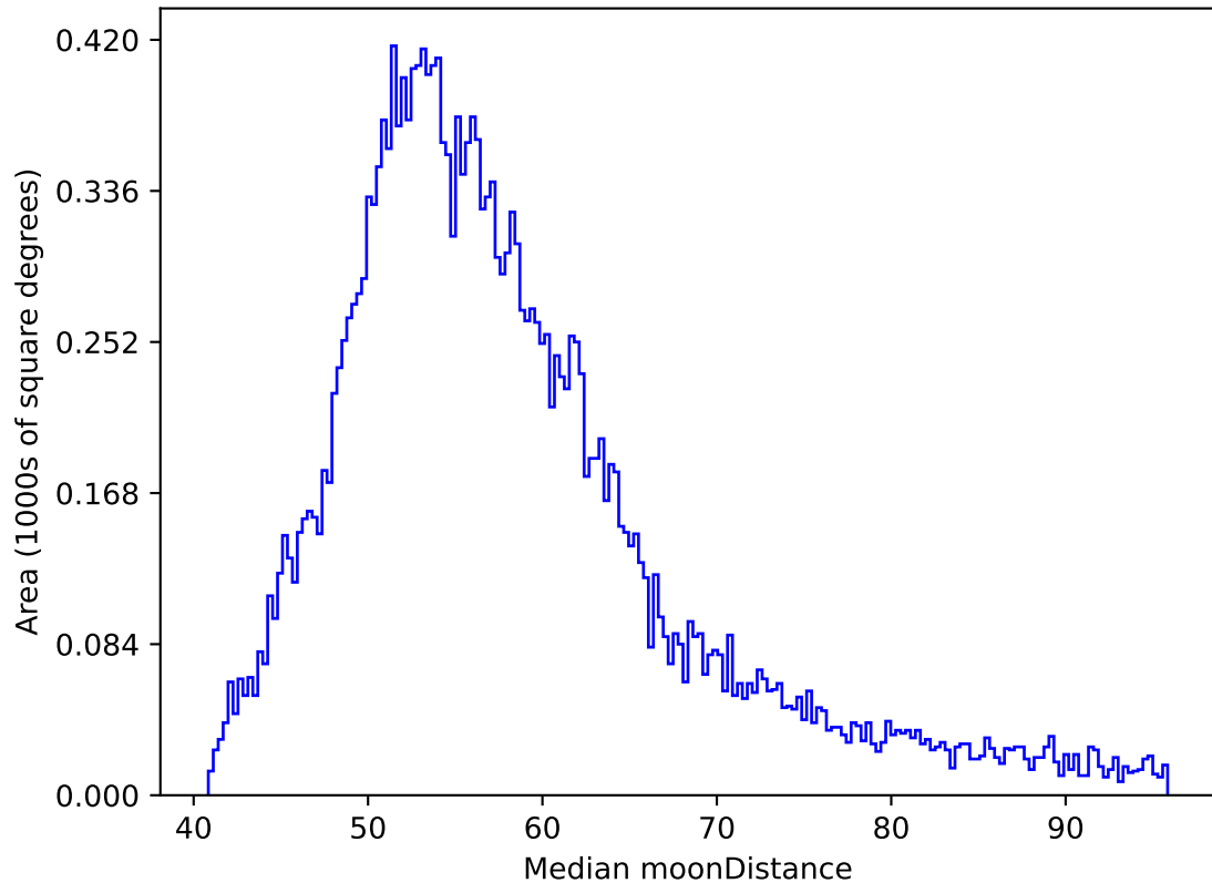
too_elab_heavy_r64_d2_ugrizy_v3.4_10yrs All sky y band: Median moonDistance
