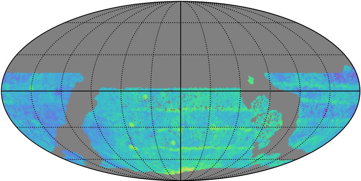
too_elab_heavy_r64_d2_ugrizy_v3.4_10yrs WFD z band: Median Season Length
