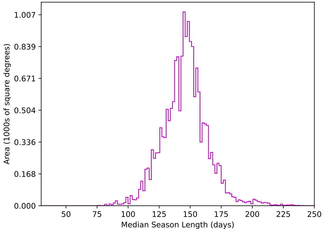
too_elab_heavy_r64_d2_ugrizy_v3.4_10yrs WFD z band: Median Season Length
