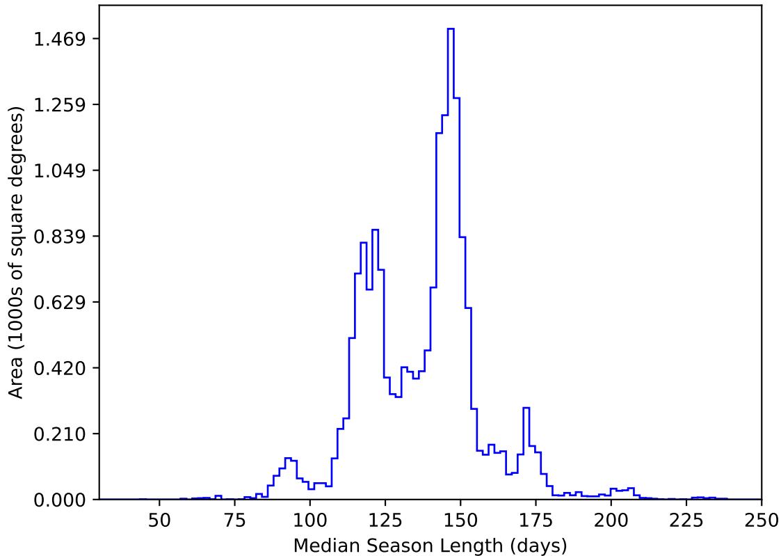
too_elab_heavy_r64_d2_ugrizy_v3.4_10yrs WFD y band: Median Season Length
