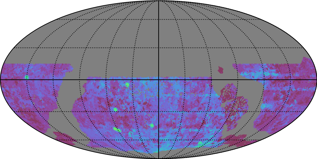
too_elab_heavy_r64_d2_ugrizy_v3.4_10yrs WFD u band: Median Season Length
