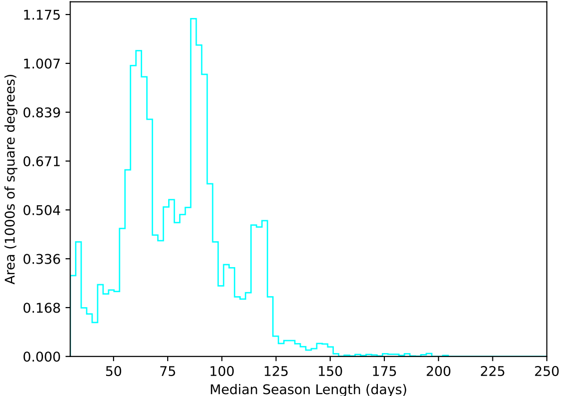
too_elab_heavy_r64_d2_ugrizy_v3.4_10yrs WFD u band: Median Season Length
