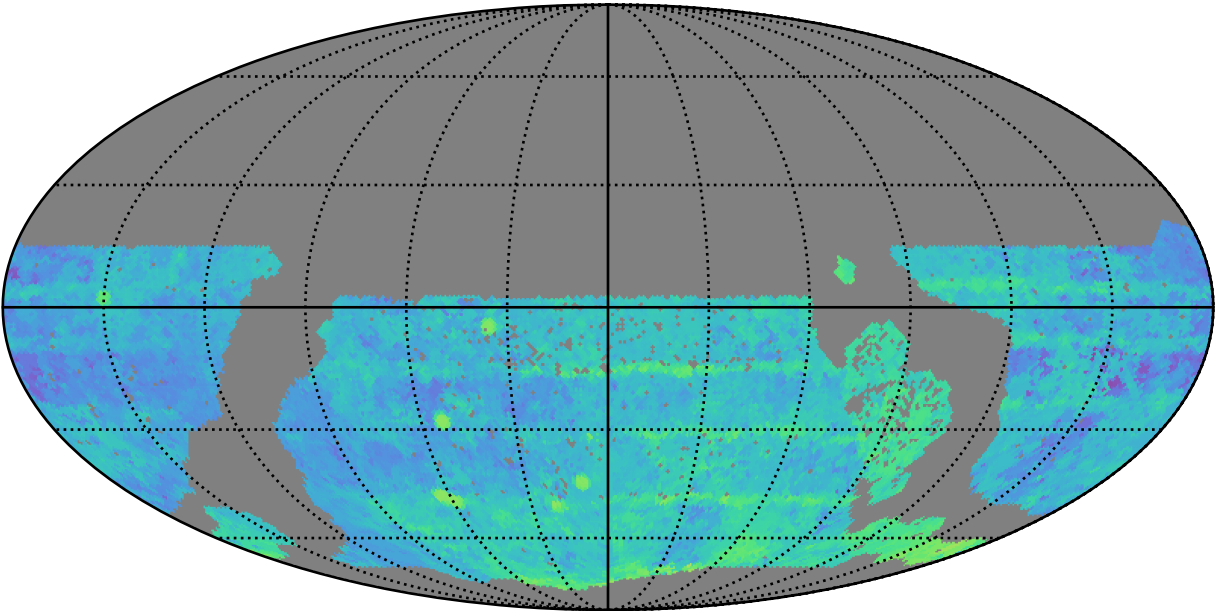
too_elab_heavy_r64_d2_ugrizy_v3.4_10yrs WFD r band: Median Season Length
