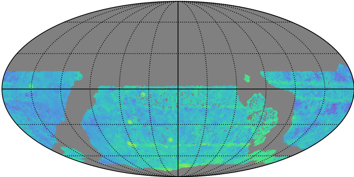
too_elab_heavy_r64_d2_ugrizy_v3.4_10yrs WFD i band: Median Season Length
