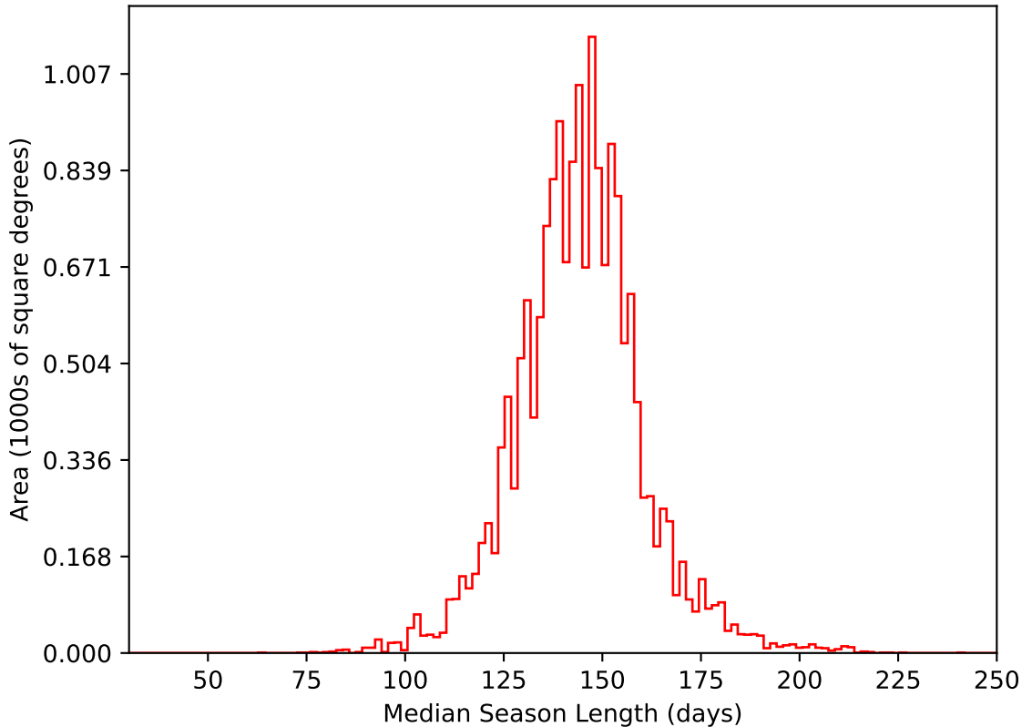
too_elab_heavy_r64_d2_ugrizy_v3.4_10yrs WFD i band: Median Season Length
