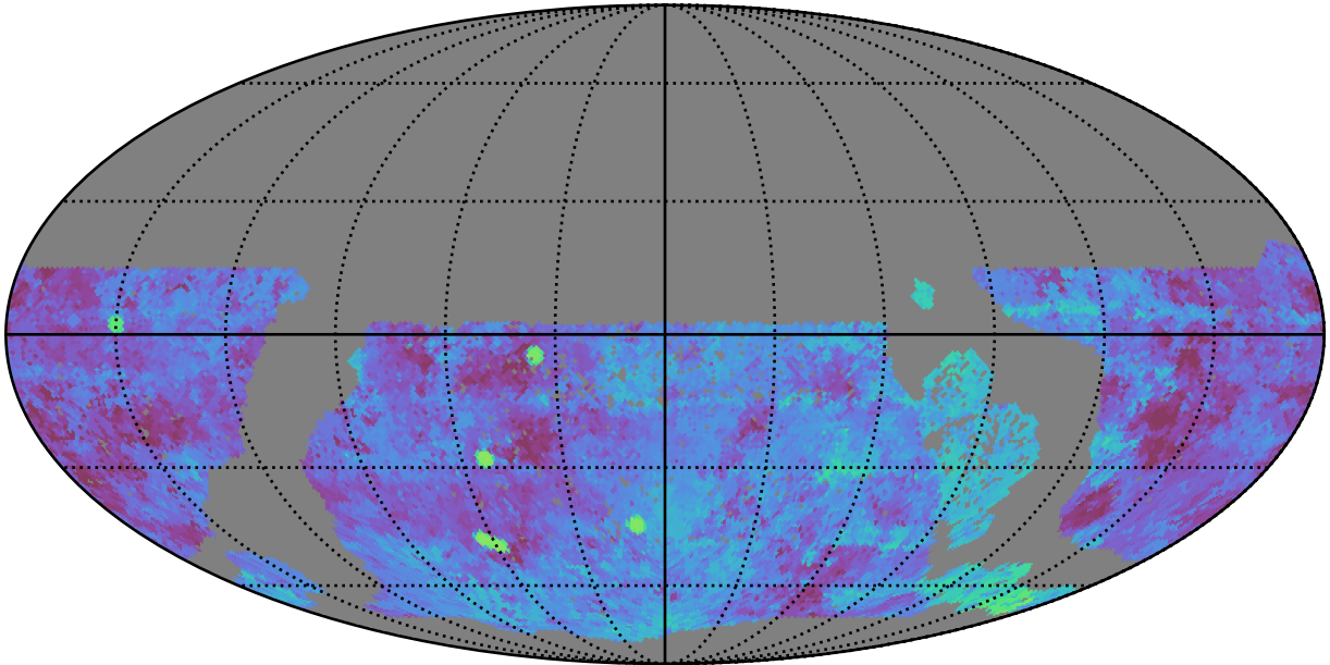
too_elab_heavy_r64_d2_ugrizy_v3.4_10yrs WFD g band: Median Season Length
