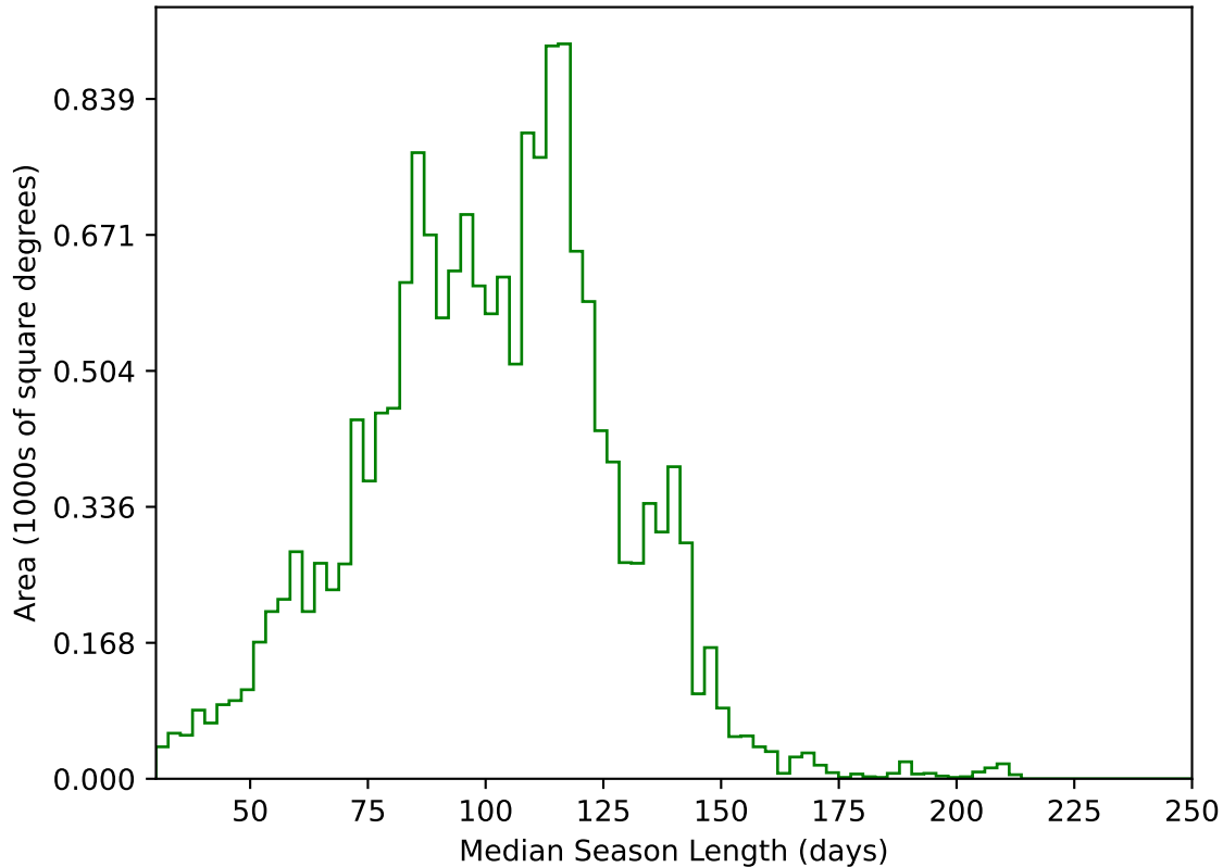
too_elab_heavy_r64_d2_ugrizy_v3.4_10yrs WFD g band: Median Season Length
