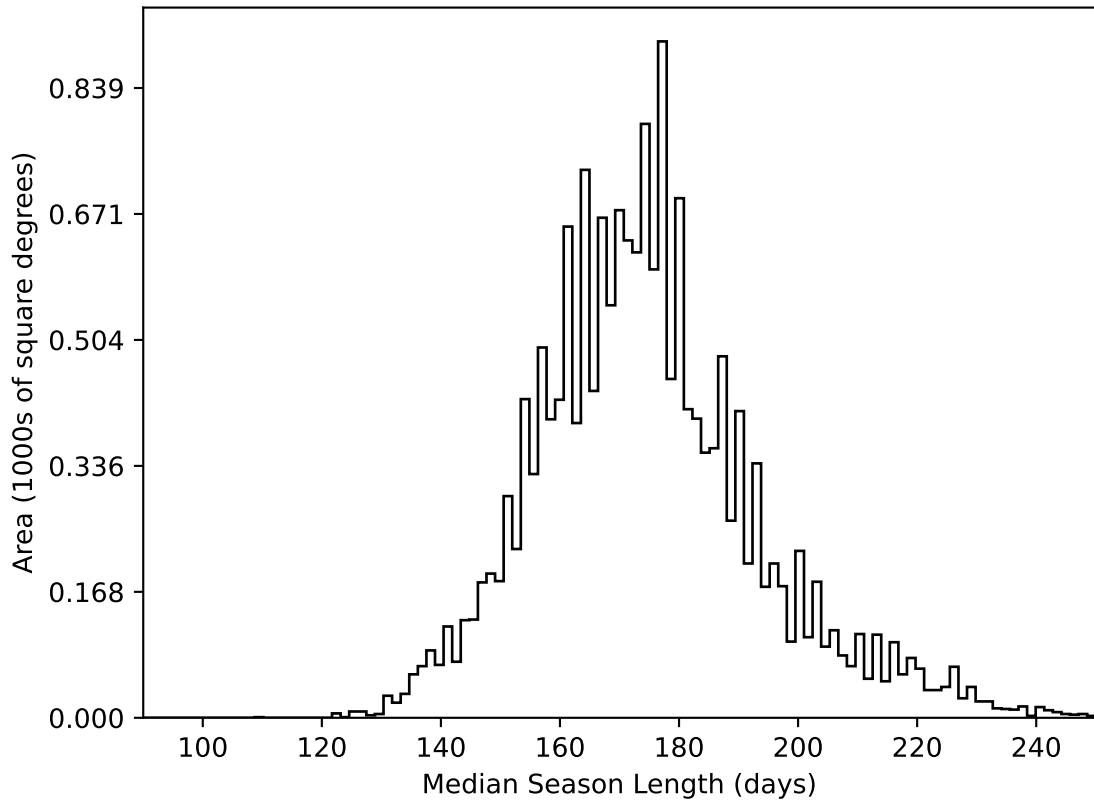
too_elab_heavy_r64_d2_ugrizy_v3.4_10yrs WFD all bands: Median Season Length
