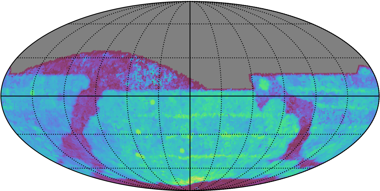
too_elab_heavy_r64_d2_ugrizy_v3.4_10yrs All sky z band: Median Season Length
