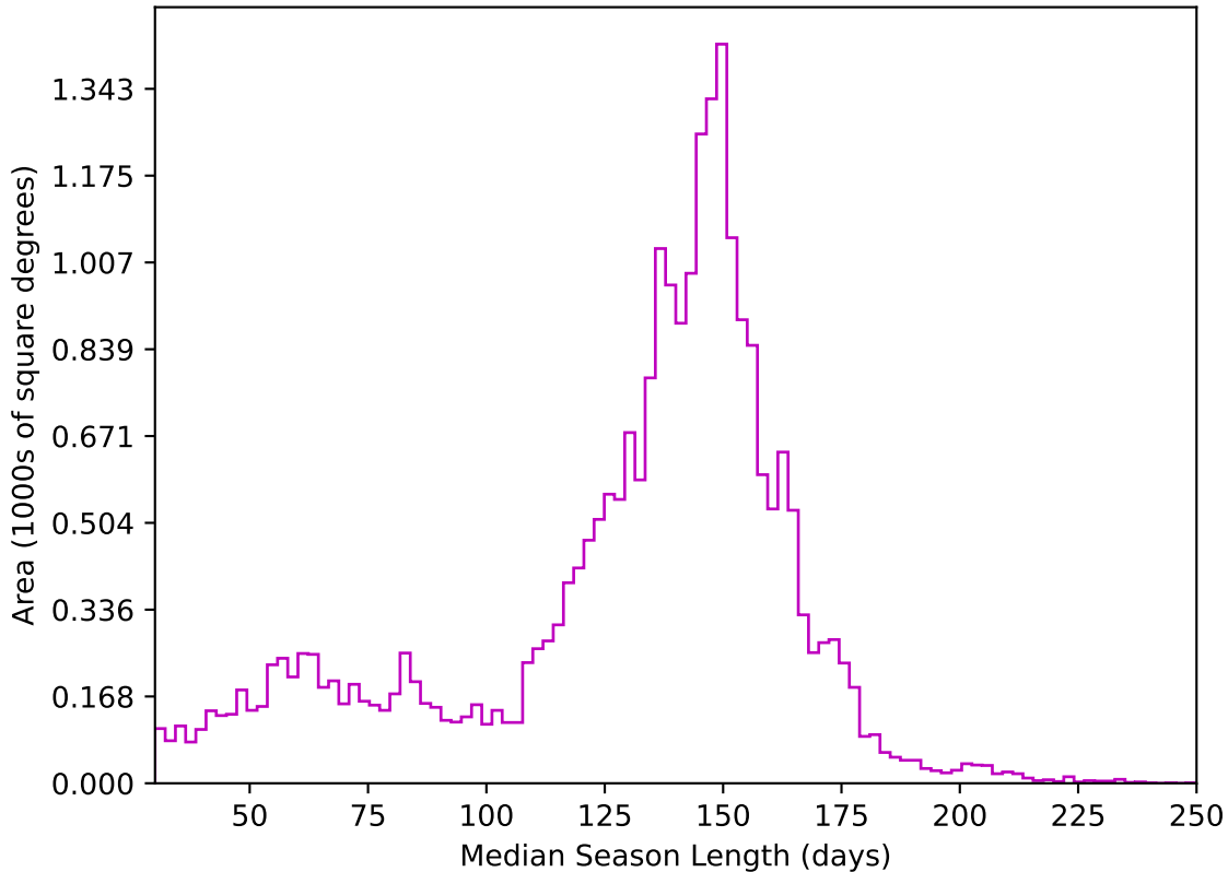
too_elab_heavy_r64_d2_ugrizy_v3.4_10yrs All sky z band: Median Season Length
