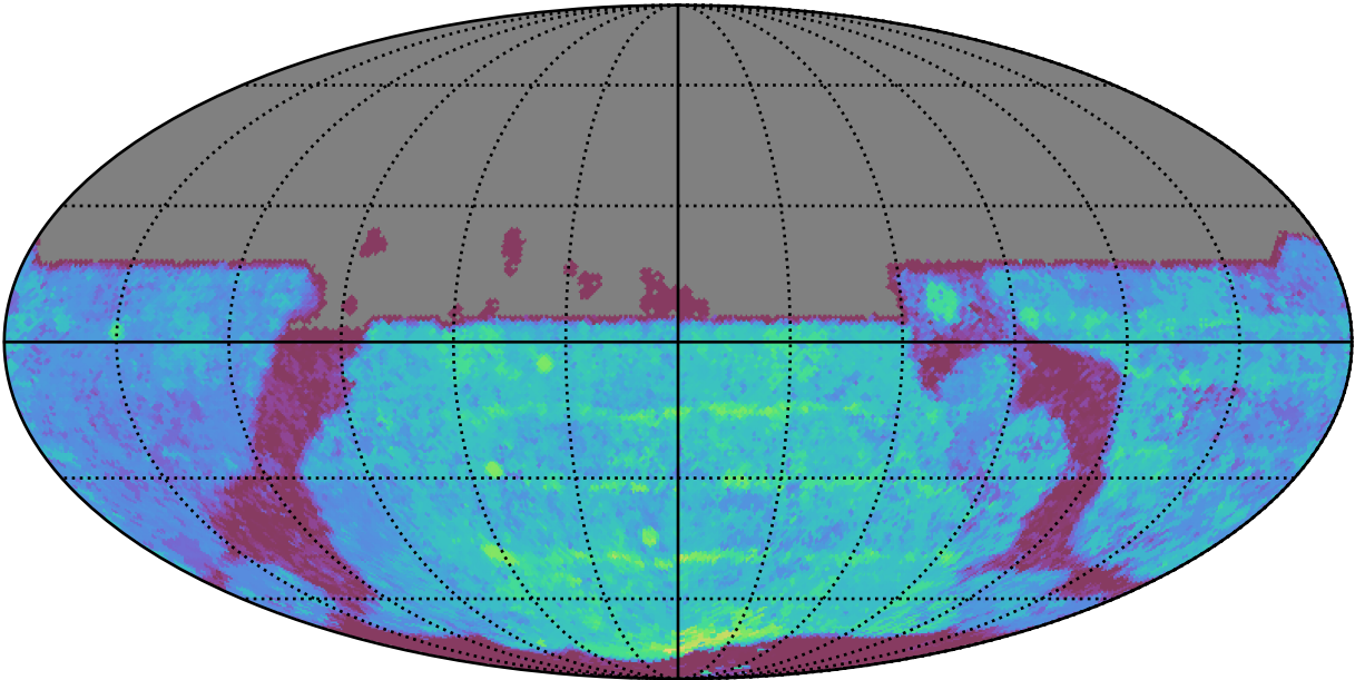
too_elab_heavy_r64_d2_ugrizy_v3.4_10yrs All sky y band: Median Season Length
