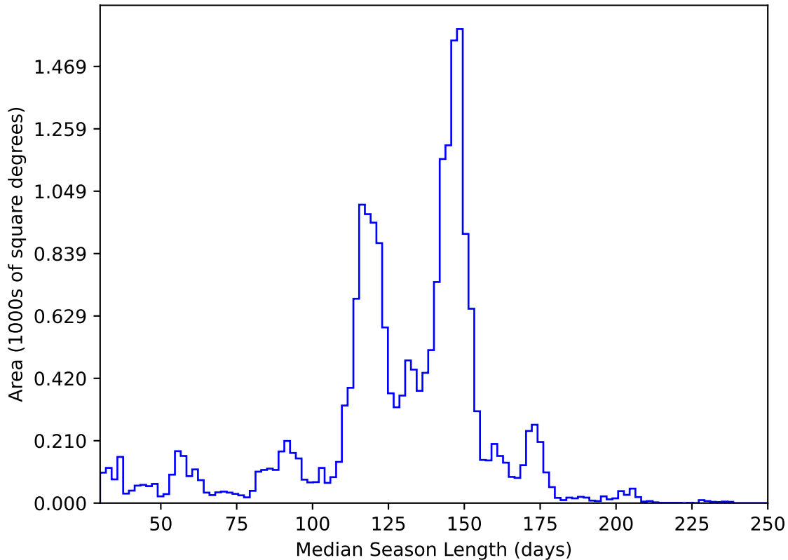
too_elab_heavy_r64_d2_ugrizy_v3.4_10yrs All sky y band: Median Season Length
