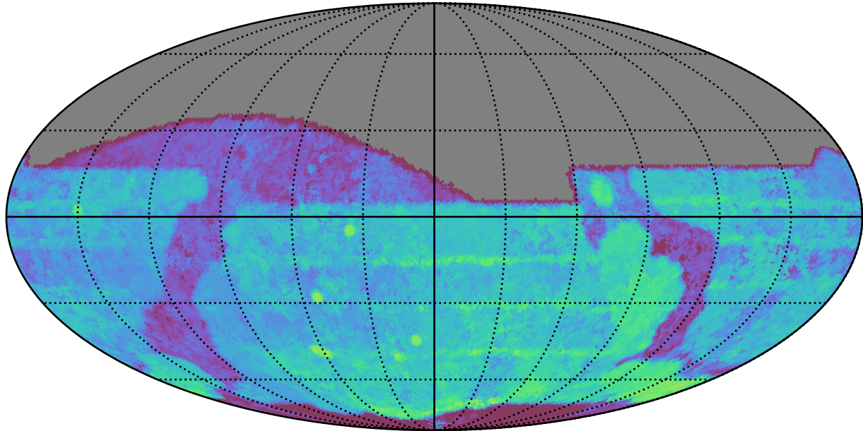
too_elab_heavy_r64_d2_ugrizy_v3.4_10yrs All sky r band: Median Season Length
