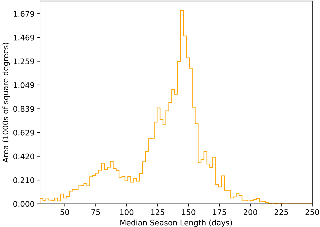
too_elab_heavy_r64_d2_ugrizy_v3.4_10yrs All sky r band: Median Season Length
