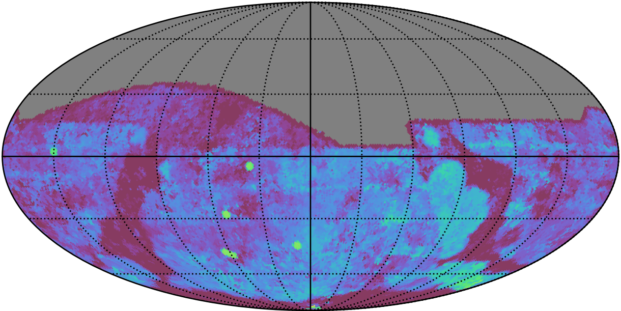
too_elab_heavy_r64_d2_ugrizy_v3.4_10yrs All sky g band: Median Season Length
